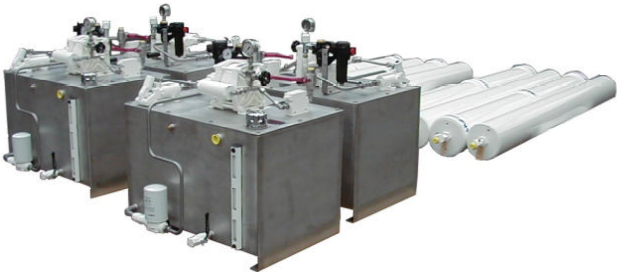
APS starting system, made out of stainless steel. The accumulators are specially painted (see water proof). All components mounted on the tank (Variation A) with the accumulators delivered as loose parts.
